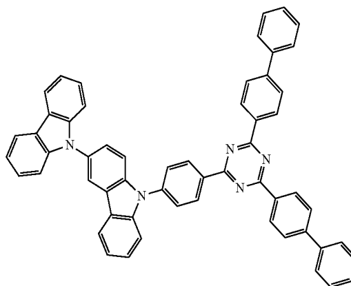
Compound 22
