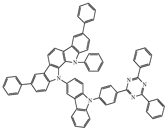
Compound 21
