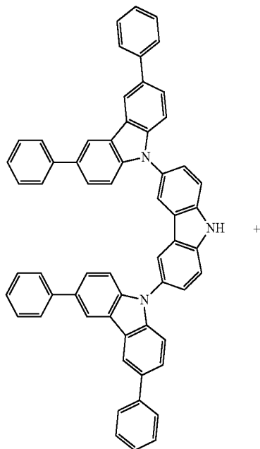
Scheme 3
