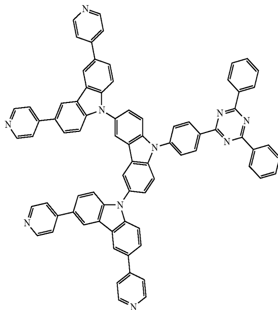
Compound 32
