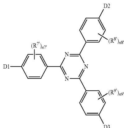
General Formula (5)
