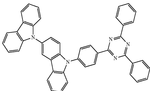
Compound 5
