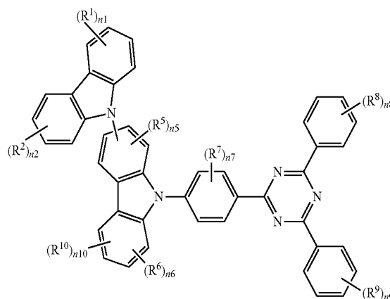
General Formula (1)
