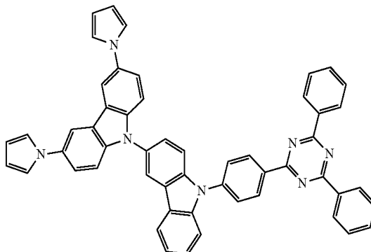
Compound 16
