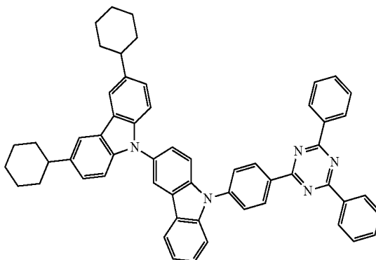
Compound 20
