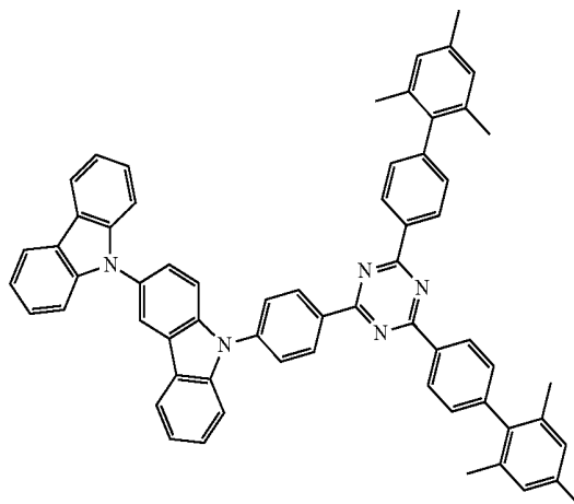
Compound 26
