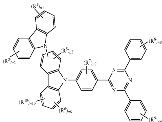
General Formula (1)
