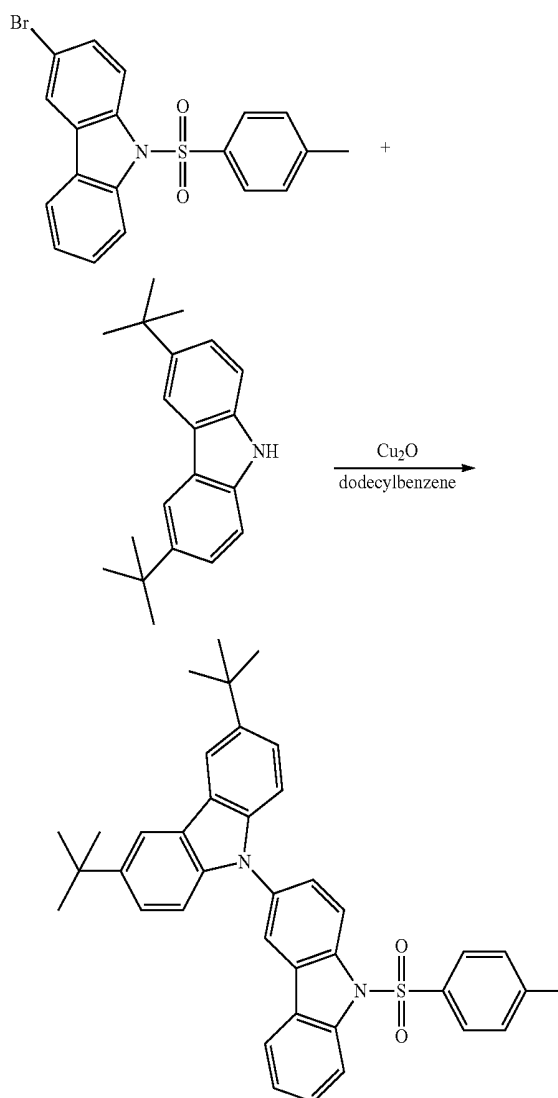
Scheme 1
