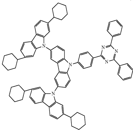
-continued Compound 47
