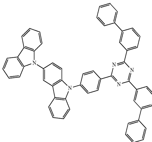
Compound 24
